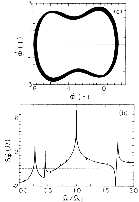
FIG. 1. Quasiperiodic regime. (a) Phase space \dot{\phi}_r(t) vs \phi(t) reveals that the quasiperiodicity corresponds to a trapped state in a number of wells of the periodic potential. (b) Voltage ( V = \dot{\phi}_r ) power spectrum S_V(\Omega) vs (\Omega/\Omega_d) makes clear the origin of quasiperiodicity: Its higher peaks correspond to the drive and breather frequencies, which are incommensurate.
